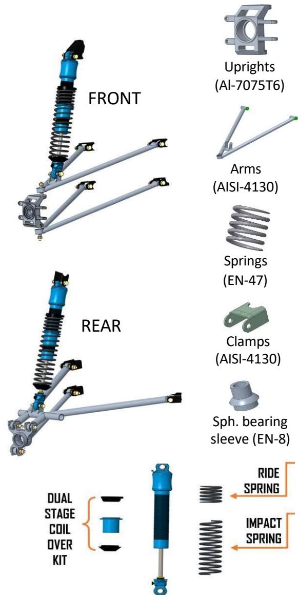
AFCD 63 SERIES 7"-3" SHOCK
